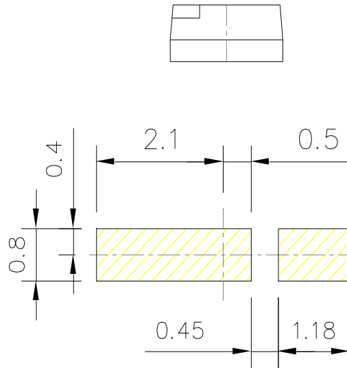
Soldering patterns
