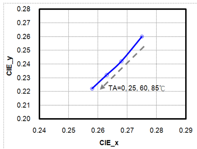
7. Chromaticity Coordinates vs. Ambient Temperature ( I_F=75\text{mA} )
